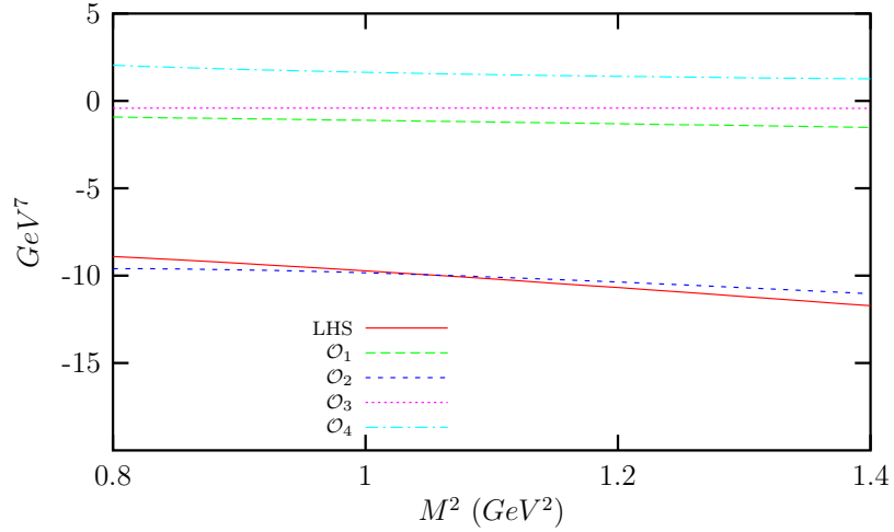
FIG. 3: The four terms on the LHS of Eq. (24) individually, together with the summation of them for s_0^q = 2.3 \text{ GeV}^2 and \chi_G \equiv \chi = -10 \text{ GeV}^{-1} . Here \mathcal{O}_1 denotes the first term, \mathcal{O}_2 denotes the second term, and so on.
