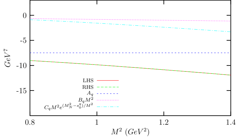
FIG. 2: (The Borel mass dependence of LHS and the fitted RHS of Eq. (24) for s_0^q = 2.3 \text{ GeV}^2 and \chi_G \equiv \chi = -10 \text{ GeV}^{-1} . We also present the terms on the RHS individually. Note that the LHS curve (solid) overlies the RHS curve (dashed).
