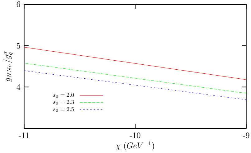
FIG. 4: The dependence of g_{NN\sigma}/g_q^\sigma on the susceptibility \chi for three different values of s_0^q = 2.0 , 2.3, and 2.5 \text{GeV}^2 ; here we take \chi \equiv \chi_G .
