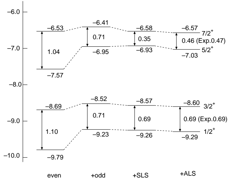
FIG. 2: Calculated energy levels of {}^7_{\Lambda}\text{Li} on the basis of \alpha + \Lambda + n + p model. The energies are measured from the \alpha + \Lambda + n + p threshold. The observed energy splittings of 3/2^+-1/2^+ and 7/2^+-5/2^+ are 0.69 MeV and 0.47 MeV, respectively.
