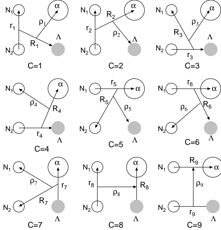
FIG. 1: Jacobian coordinates for all the rearrangement channels ( c = 1 \sim 9 ) of the \alpha + \Lambda + n + p four-body model. Two nucleons are to be antisymmetrized.
