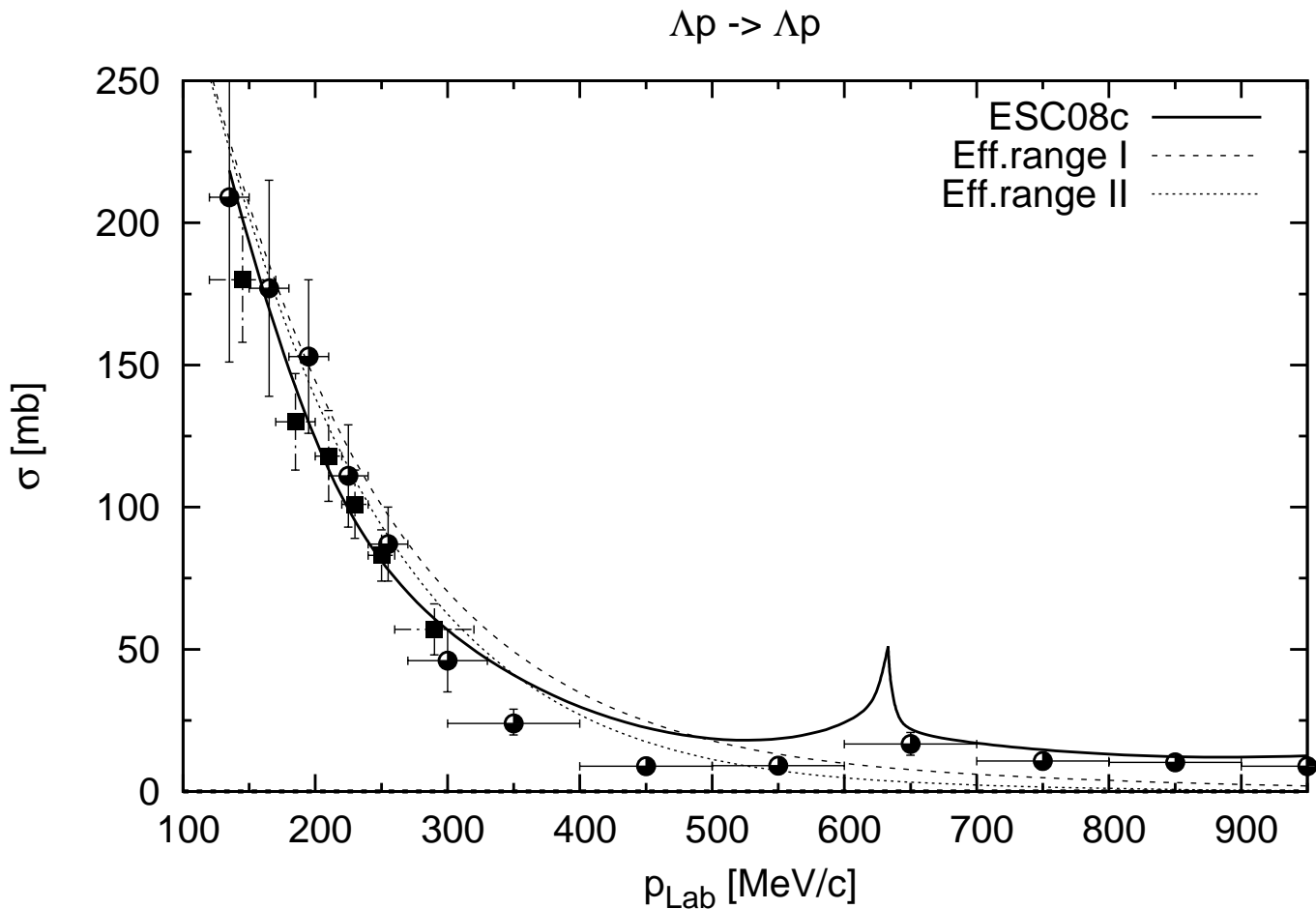
FIG. 1: Model fits total X-sections \Lambda p . Rehovoth-Heidelberg-, Maryland-, and Berkeley-data
