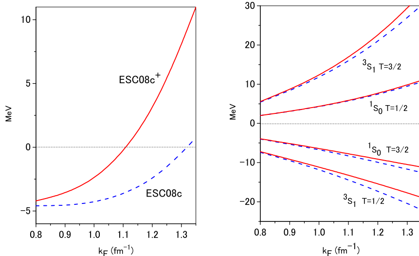
FIG. 7: In the left (right) panel, the values of U_\Sigma (partial-wave contributions) are drawn as a function of k_F by dashed and solid curves for ESC08c and ESC08c + , respectively.
