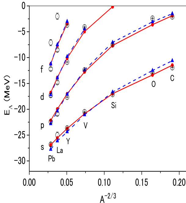
FIG. 6: Energy spectra of ^{13}_{\Lambda}\text{C} , ^{28}_{\Lambda}\text{Si} , ^{51}_{\Lambda}\text{V} , ^{89}_{\Lambda}\text{Y} , ^{139}_{\Lambda}\text{La} and ^{208}_{\Lambda}\text{Pb} are given as a function of A^{-2/3} , A being mass numbers of core nuclei. Solid (dashed) lines show calculated values by the G-matrix folding model derived from ESC08c + (ESC08c). Open circles denote the experimental values taken from Ref. [60].
