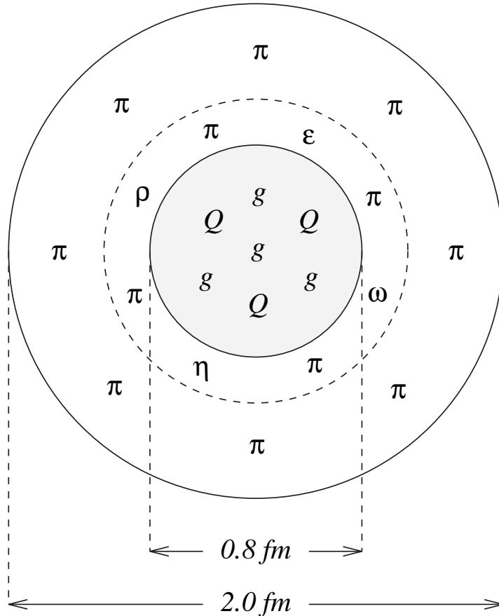
FIG. 1. Schematic model of the baryon structure
