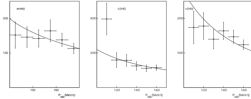
FIG. 4. The total elastic cross sections \Sigma^-p \rightarrow \Sigma^-p and the charge exchange reactions \Sigma^-p \rightarrow \Sigma^0n and \Sigma^-p \rightarrow \Lambda^0n [21, 22].
