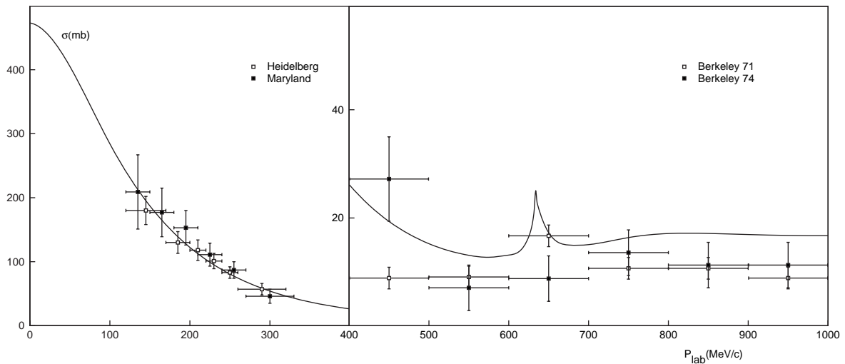
FIG. 2. Cross sections for elastic \Lambda p scattering. The data are taken from [17, 18, 19, 20].
