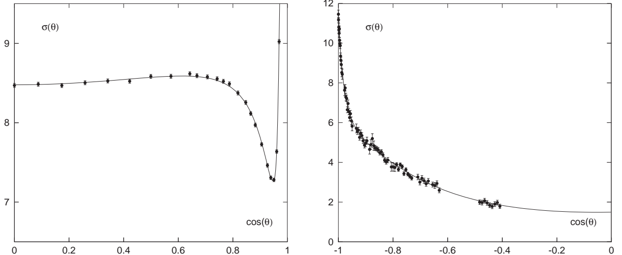
FIG. 1. (a) pp differential cross section at 50.06 MeV [12]. The 24 datapoints contribute \chi^2 = 12.8 in the Nijm PWA93. (b) np backwards differential cross section at 344.3 MeV [13]. The 80 datapoints contribute \chi^2 = 74.53 to the Nijm PWA93 and have the normalization 1.035 \pm .005 .
