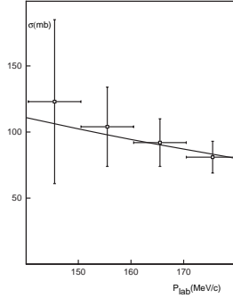
FIG. 3. The \Sigma^+p elastic total cross section [21].
