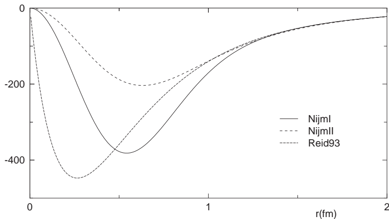
FIG. 1. The tensor potential connecting the {}^3S_1 and {}^3D_1 partial waves.
