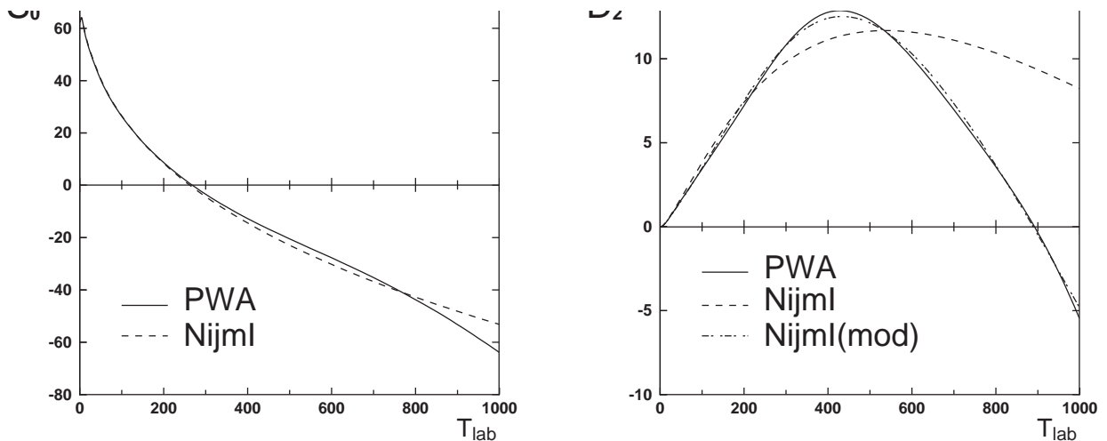
FIG. 4. ^1S_0 and ^1D_2 phase shifts for the optical Nijm I potential and for the modified version.
