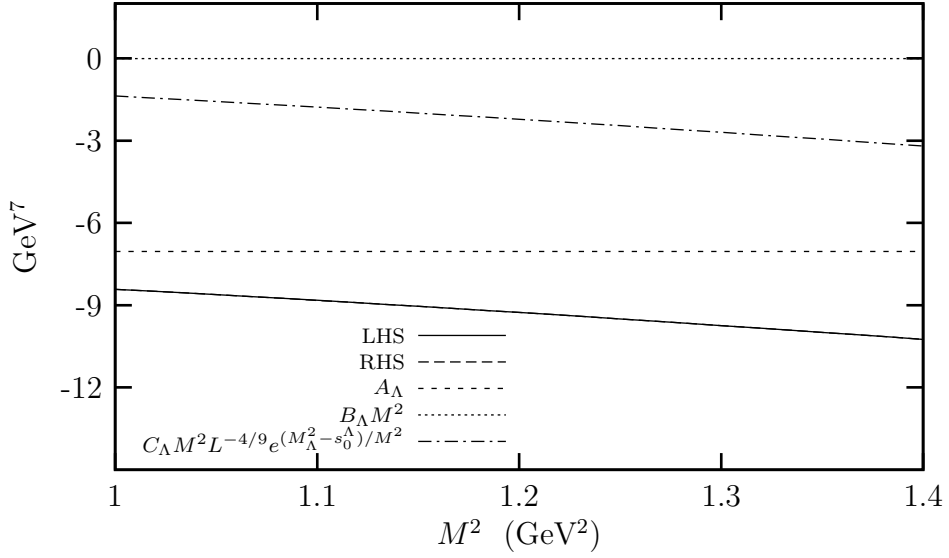
FIG. 6: The Borel mass dependence of LHS and the fitted RHS of the sum rule for \Lambda\Lambda\sigma coupling in Eq. (25) with the SU(3) breaking effects and for \chi_G \equiv \chi = -10 \text{ GeV}^{-1} . We also present the terms on the RHS individually. Note that the LHS curve (solid) overlies the RHS curve (dashed).
